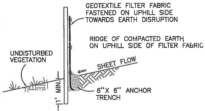
SECTION VIEW
