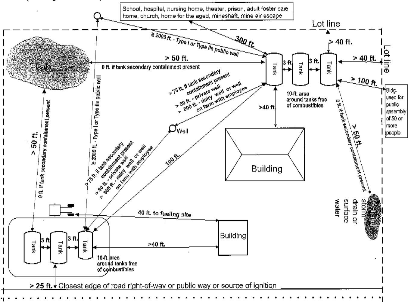
Figure 2. Aboveground small ( \leq 1,100 gallons) UL 142 tank separation distances. All measurements should be considered minimum. (Drawing not to scale.)
